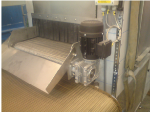
Tunnel washer with transport mat
