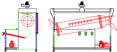
Tunnel with screw-feeder
