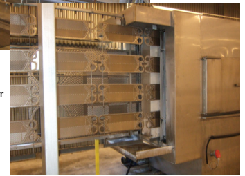
Tunnel washer with hanging conveyor
