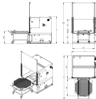
Layout simplex big, 1-tank.
