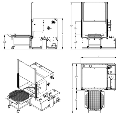
Layout simplex big, 2-tanks.
