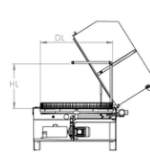
Lay out P100/ P120/100LT/120LT/100HT/120HT
