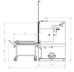
Layout simplex big, 1-tank.
